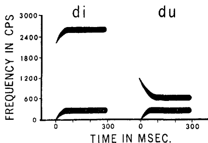
FIG. 1. Spectrographic patterns sufficient for the synthesis of /d/ before /i/ and /u/.
