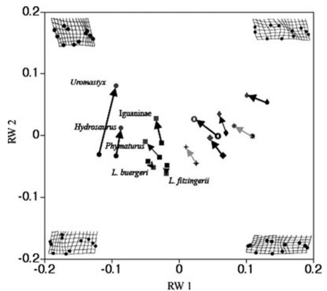
Figure 5. Convergent evolutionary changes may not erase differences among clades. In lizards, the evolution of herbivory usually leads to evolutionary change in morphology in the same direction, as indicated by the direction of the vector. However, these changes are not sufficient to override among-clade differences. Axes represent different aspects of head morphology, as analyzed using geometric morphometric methods. Figure from Stayton (2006).
