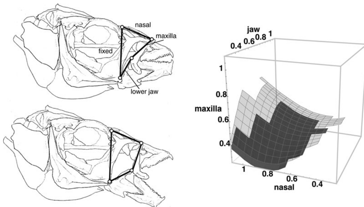
Figure 3. Many-to-one morphology-to-performance mapping. Labrid fish have highly kinetic heads and jaw protrusion is affected by four linked bony elements. The three-dimensional surface illustrates the different combinations of jaw, maxilla, and nasal length (all scaled in proportion to the positionally fixed head element) that produce the same biomechanical performance in jaw protrusion. Figure on left from Wainwright et al. (2005); figure on right from Alfaro et al. (2005).
