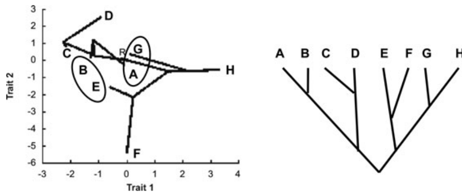
Figure 1. Convergence resulting from random evolution. In a simulation, traits evolved according to Brownian motion and speciation occurred according to a pure-birth Yule process of cladogenesis (Stayton 2008). The result is that some species evolved to become more phenotypically similar than were their ancestors (e.g., species A and G, and B and E). R represents the phenotype of the ancestor (root). Figure modified from Stayton (2008).
