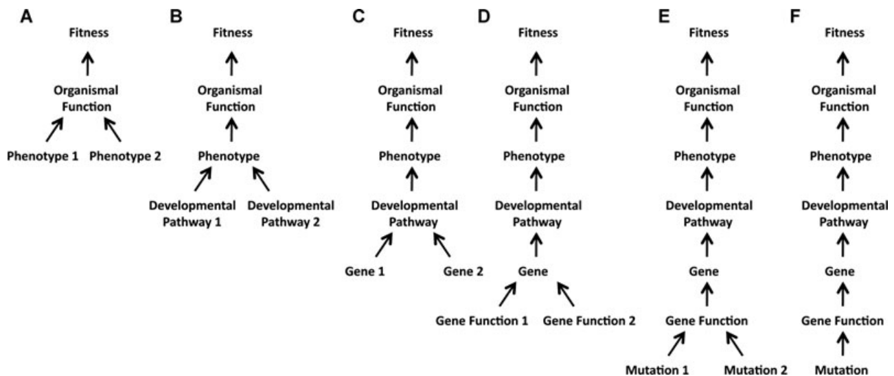
Figure 6. Nonconvergence at lower hierarchical levels produces convergence at higher levels. (A) Many-to-one mapping of performance to morphology results in convergence in performance, but not in phenotype; (B) nonconvergent developmental changes produce convergent phenotypes; (C) mutations in different genes produce convergent changes in development; (D) different functional changes within the same gene produce convergent change in development; (E) different mutations in the same gene produce convergent change in gene function; (F) convergent mutational change produces convergent changes at all hierarchical levels.
