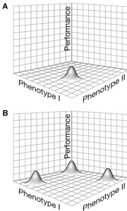
Figure 4. Many-to-one morphology-performance relationships and convergence. (A) If there is a direct, linear relationship between morphology and performance, then selection for a particular performance ability will lead to convergent evolution of similar morphology in multiple taxa. (B) By contrast, when many-to-one relationships exist, then convergent evolution in performance capability may occur by nonconvergent evolution of morphology. From Losos (2009).
