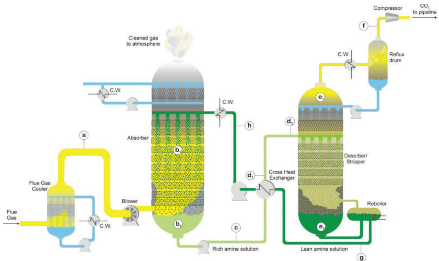
Figure 28: Amine CCS Process Flow Diagram
